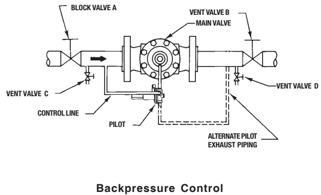
Figure 5. Backpressure Regulator/Relief Valve Applications
