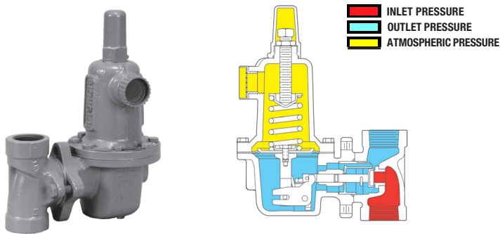
Figure 1. Type 627 Direct-Operated Regulator and Operational Schematic
