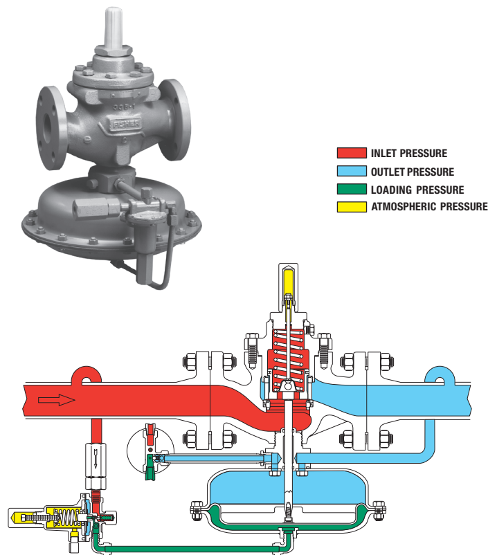
Figure 2. Type 1098-EGR Pilot-Operated Regulator and Operational Schematic
