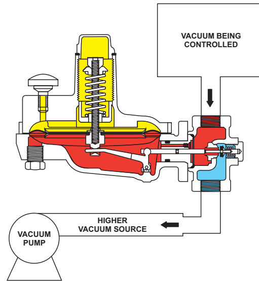
Figure 4. Type Y690VB Vacuum Breaker and Type V695VR Vacuum Regulator Operational Schematics
