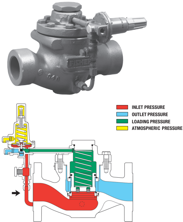
Figure 3. Type 63-EG Backpressure Regulator/Relief Valve and Operational Schematic
